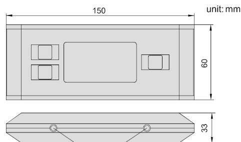
Magnetic base
