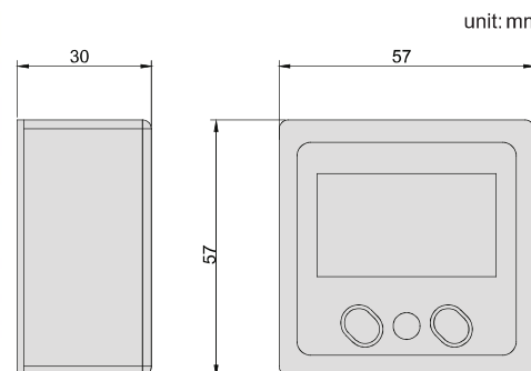
Magnetic base
